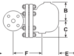
FT44 DN25, DN40 and DN50
